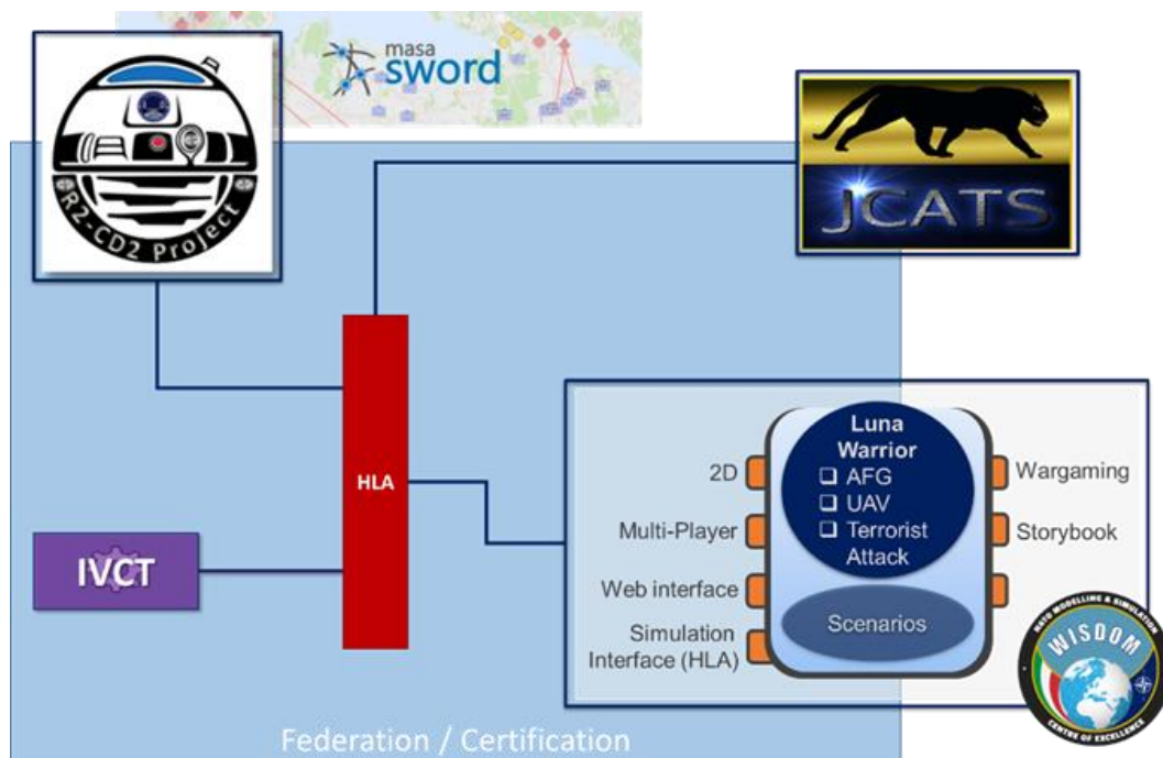
Figure 5 Scatch of a wargaming and simulation integration activity by federating WISDOM with simulation systems
